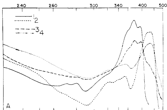
Fig. 2.—Ultraviolet absorption of salicylaldehyde derivatives: 1, 2,5-bis-( o -hydroxyphenyl)-thiazolo[5,4-d]thiazole (V); 2, sodium salt of (1); 3, bis-salicylidenedithiooxamide (VII); 4, sodium salt of (3), freshly prepared; solutions 2 \times 10^{-5} molar, in ethanol + 10% chloroform.
