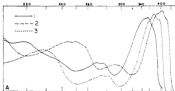
Fig. 1.—Ultraviolet absorption of thiazolo[5,4-d]thiazoles (V): 1, 2,5-diphenyl; 2, 2,5-bis-(2-furyl); 3, 2,5-bis-(β-styryl); solutions 2 \times 10^{-3} molar in ethanol (for others, see Table II).
